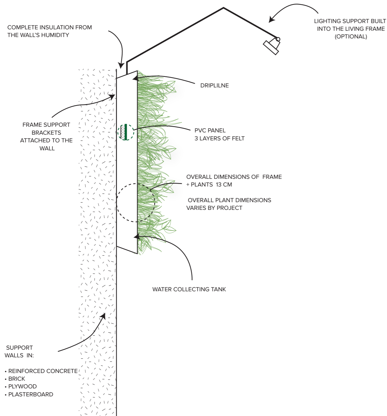
SIDE VIEW
